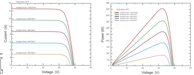
Current-Voltage & Power-Voltage Curves (SKT455M10-108D6)
